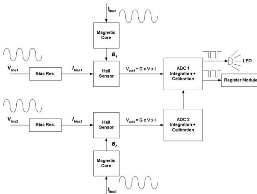
Figure 15: Hall Cells and ADCs
