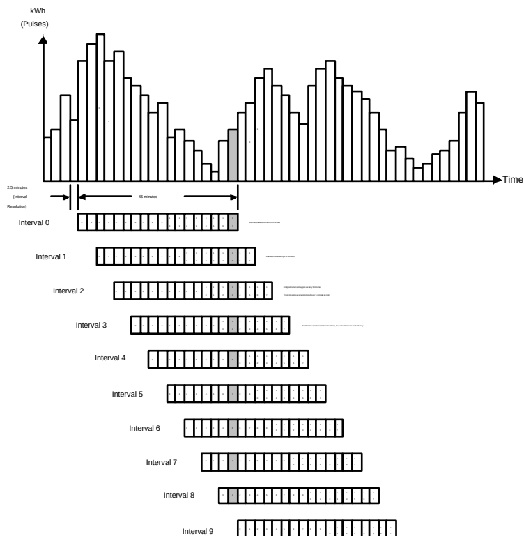
Figure 29: Cellnet Telemetry
