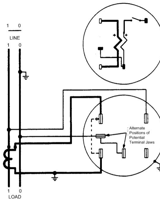
Figure 38: Form 2S Wiring Diagram
