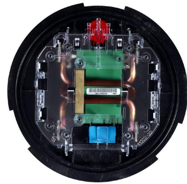
Figure 3: CENTRON 240 Volt Metrology
