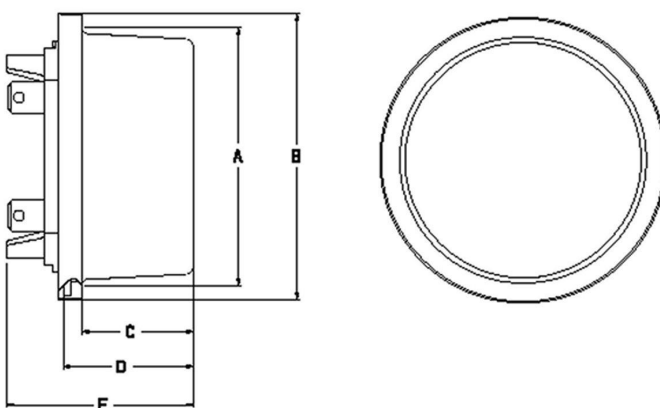
Figure 6: Dimensions
