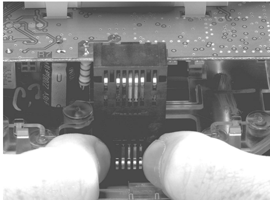
Figure 11: Board-to-Board Connector, Bottom
