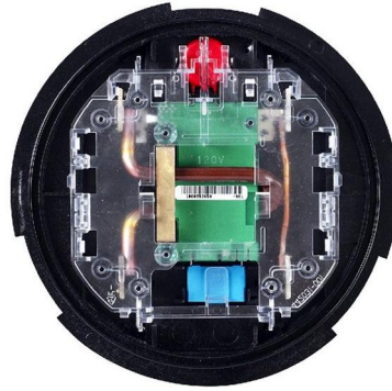
Figure 2: CENTRON 120 Volt Metrology
